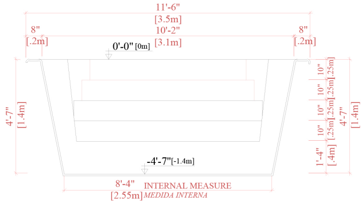
CROSS SECTION CORTE TRANSVERSAL
