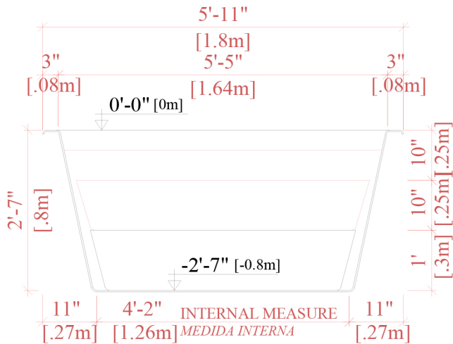
CROSS SECTION CORTE TRANSVERSAL
